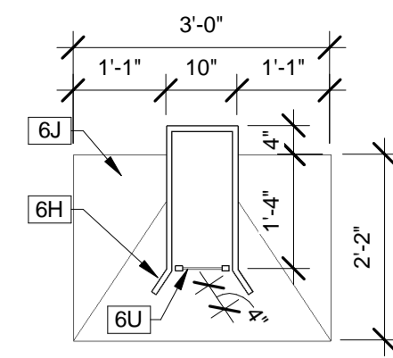
12 DESK PLAN/SECTION 1/2" = 1'-0"
