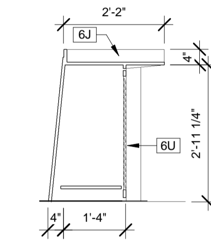
09 DESK SECTION 1/2" = 1'-0"
