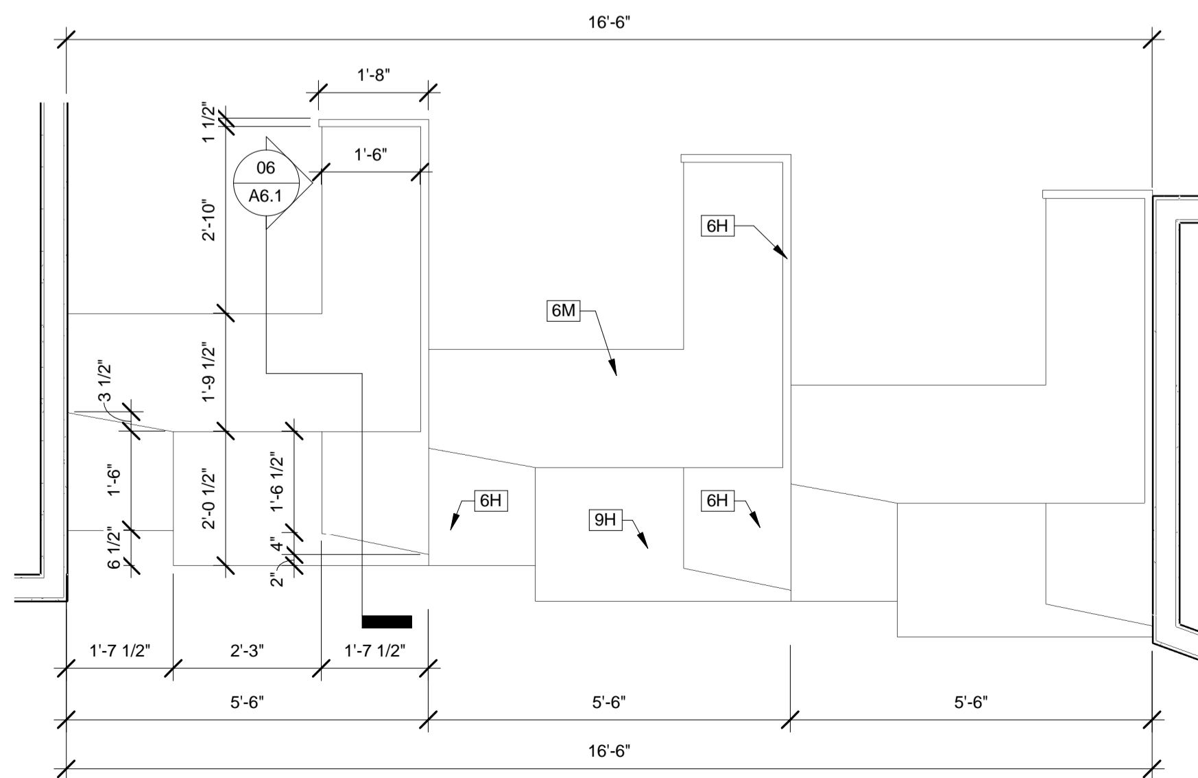
02 ENLARGED TELLER LINE PLAN 1/2" = 1'-0"
