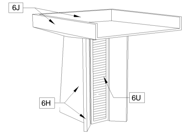
08 DESK PERSPECTIVE 1/2" = 1'-0"
