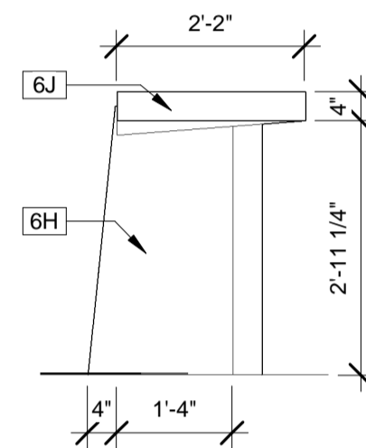
10 DESK ELEVATION - SIDE 1/2" = 1'-0"
