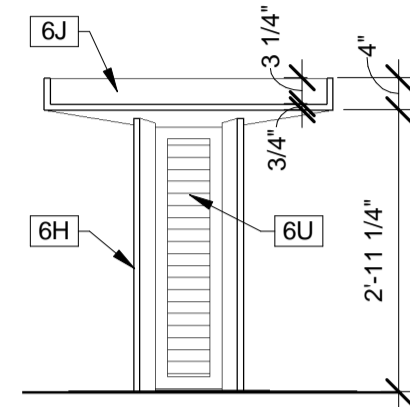
11 DESK ELEVATION - FRONT 1/2" = 1'-0"
