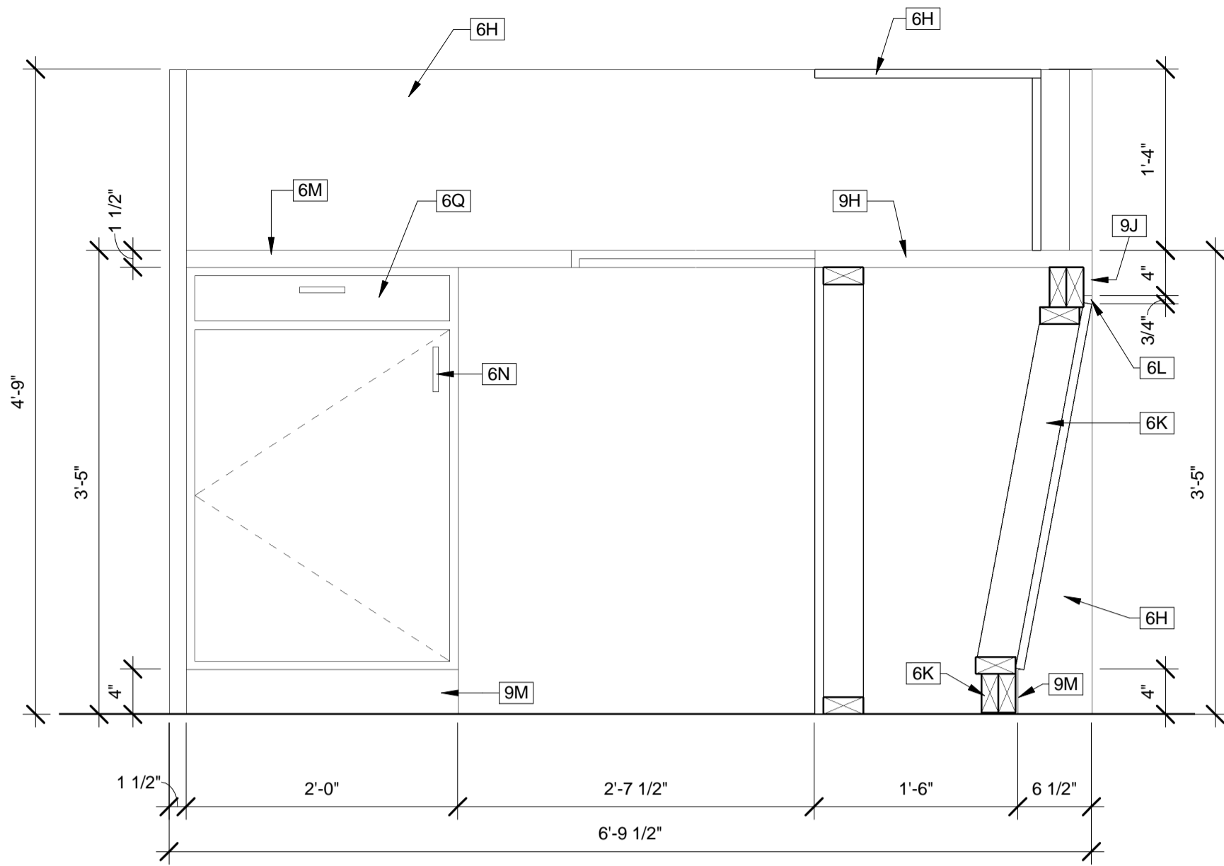
06 TELLER LINE DESK DETAIL 1" = 1'-0"
