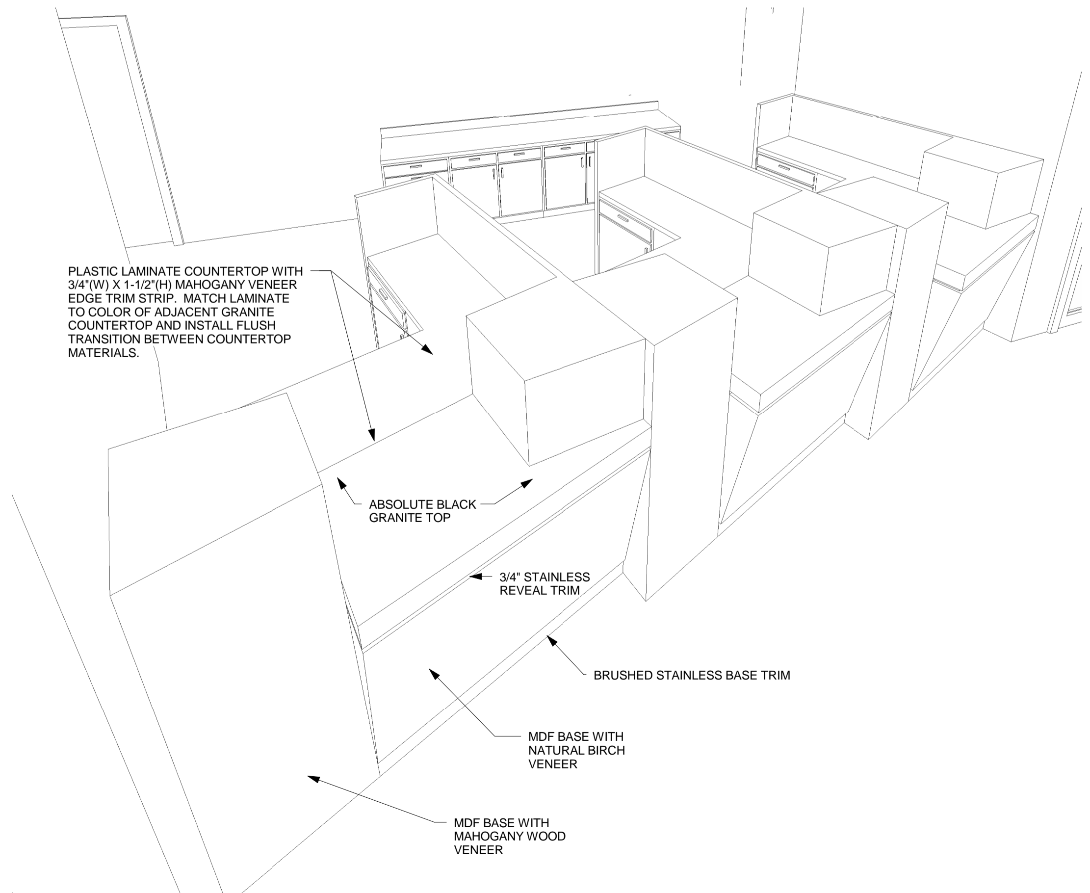
01 TELLER LINE PERSPECTIVE
