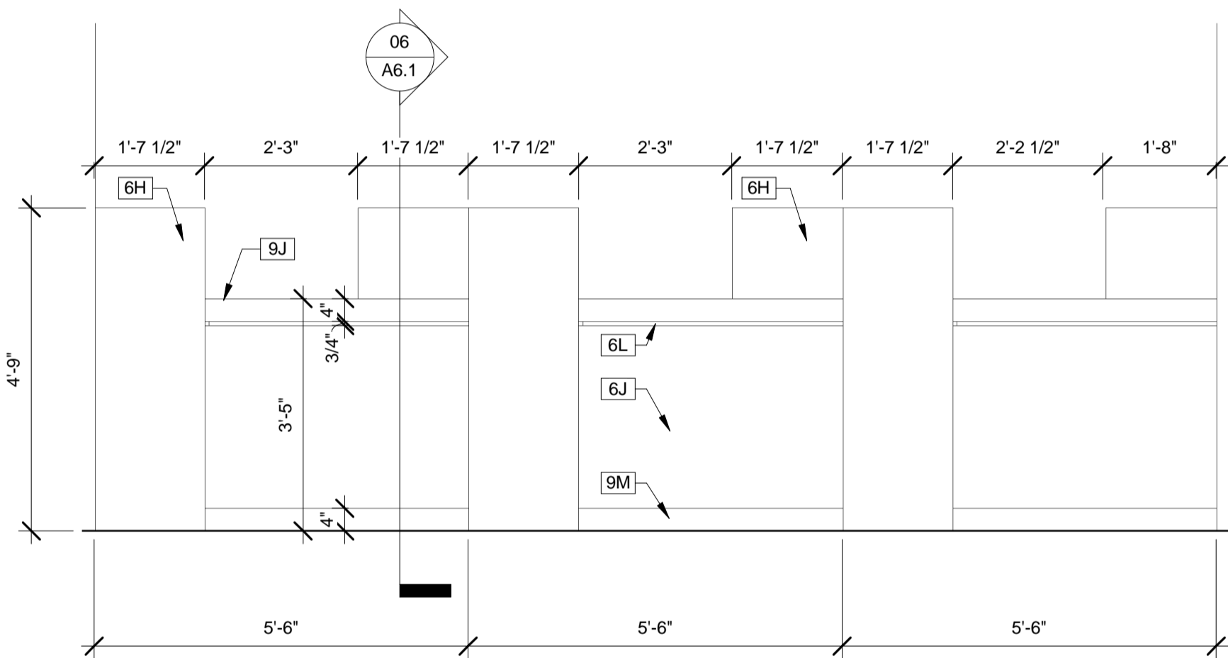
04 LOBBY 101 A 1/2" = 1'-0"
